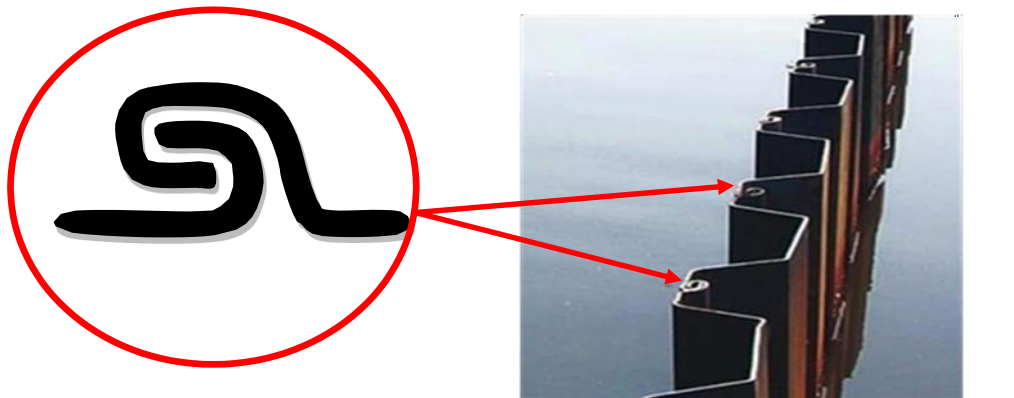
Fig.2 Various applications of steel sheet pile
