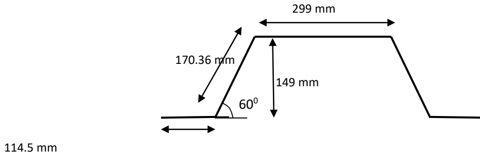
Fig.7 Sheet pile cross section used for analysis of joints
