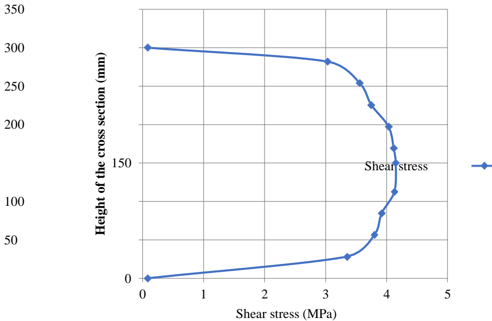
Fig.11 Height of cross section v/s shear stress for Z profile sheet pile
